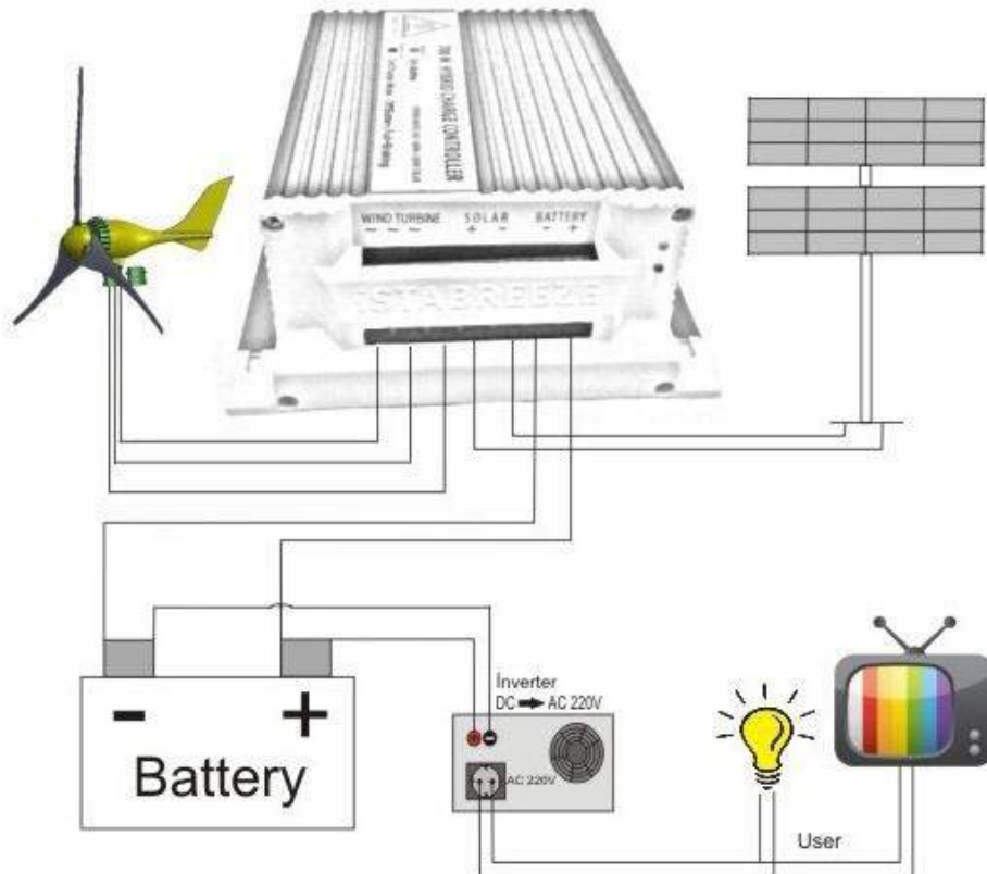
Wiring diagram for an example
