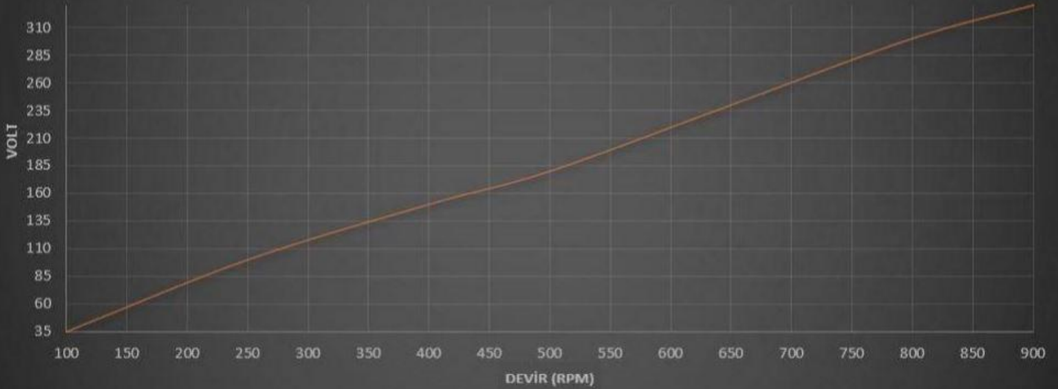
Heli-4kW-48V-Generator-Rpm-Volt-Graphic
