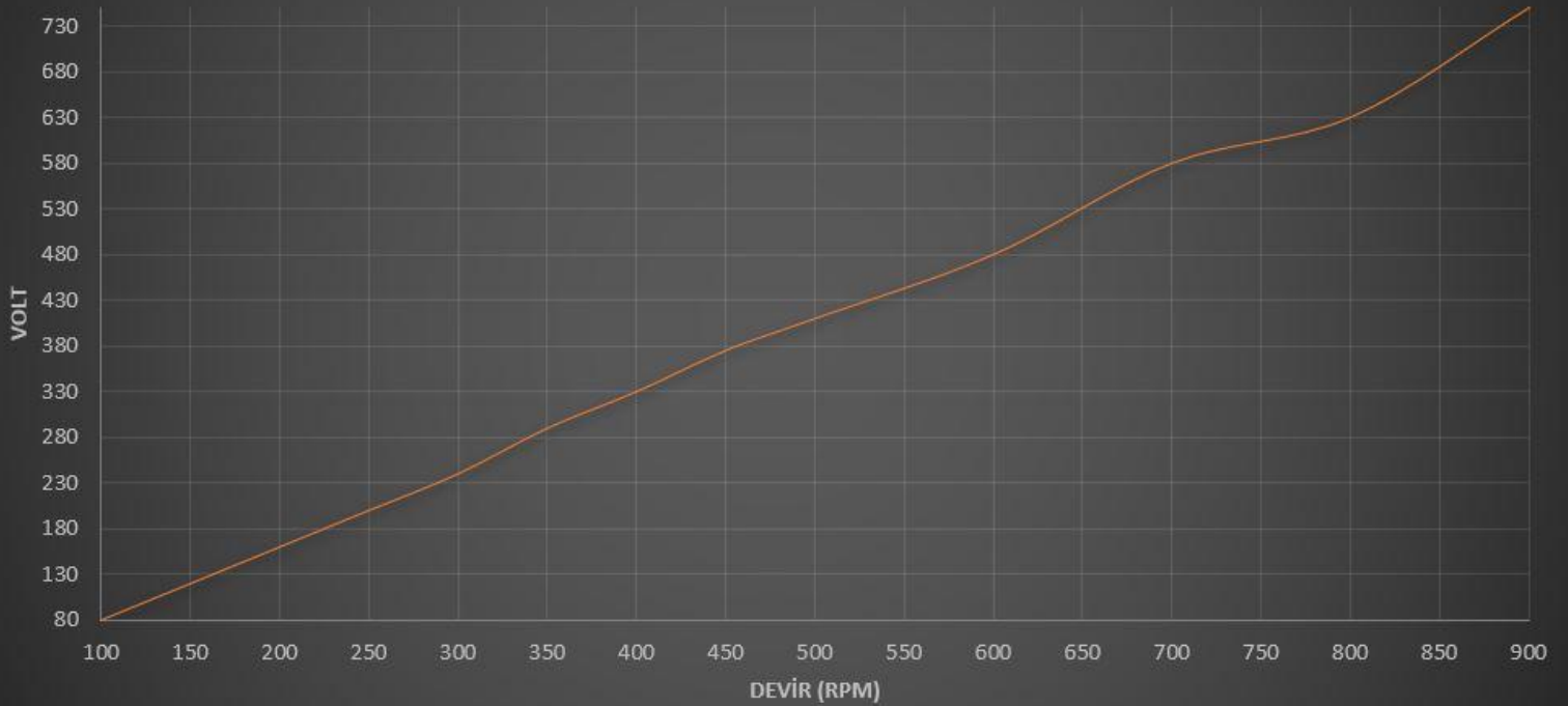
Heli-4kW-Ongrid-Generator-Rpm-Volt-Graphic
