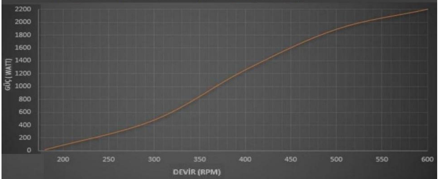
Heli-2kW-Generator-Rpm-Power-Graphic
