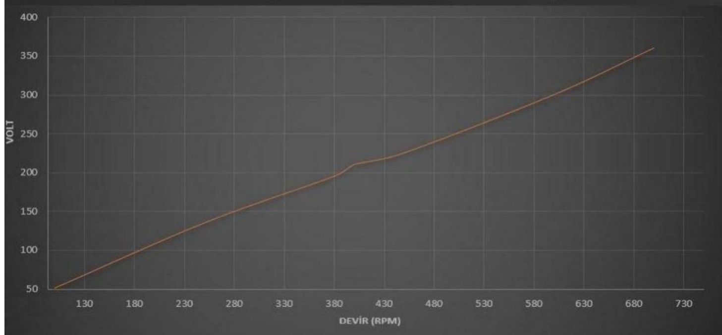
Heli-2kW-Ongrid-Generator-Rpm-Volt-Graphic
