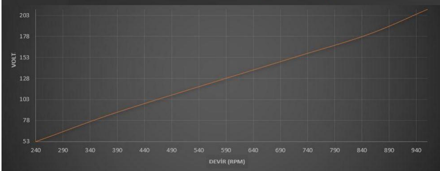
Heli-2kW-Ongrid-Generator-Rpm-Volt-Graphic
