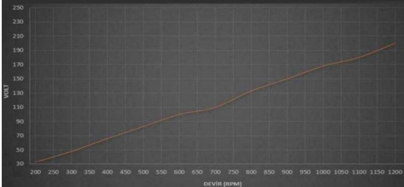
2000G-48V-Generator-Rpm-Volt-Graphic
