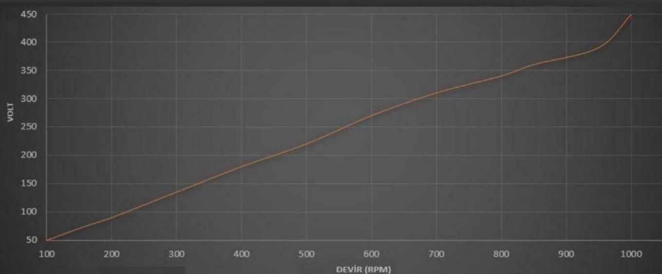
2000G-Ongrid-Generator-Rpm-Volt-Graphic
