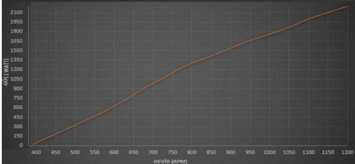
2000G-Generator-Rpm-Power-Graphic
